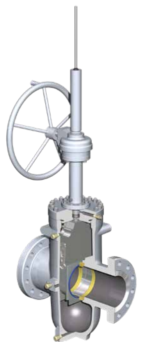
Gate Valve
