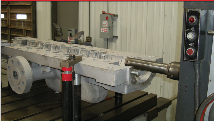
MULTI-STAGE CASE REPAIRS
